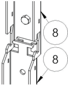
Step 3: Stacking VH-003 units in series
