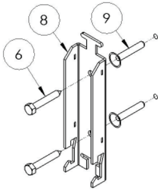
Step 2: Mounting the wall plate
