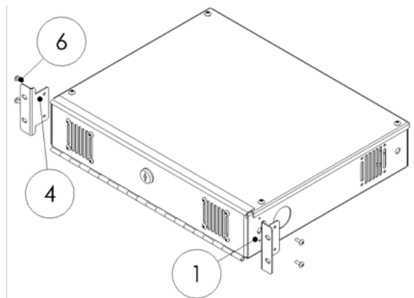
Step 6: Attaching the Ears to the Bottom Box
