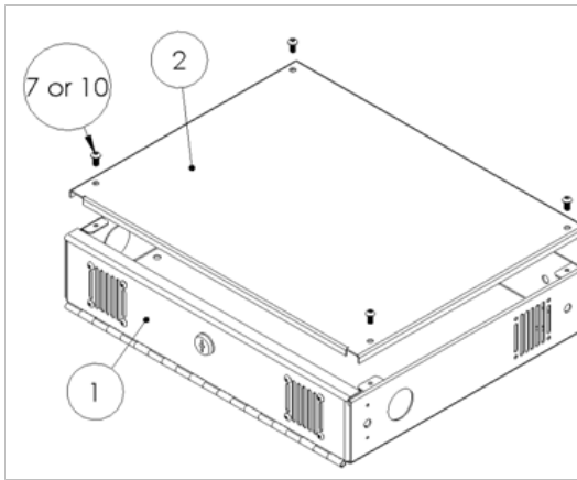
Step 8: Removing the Top Lid
