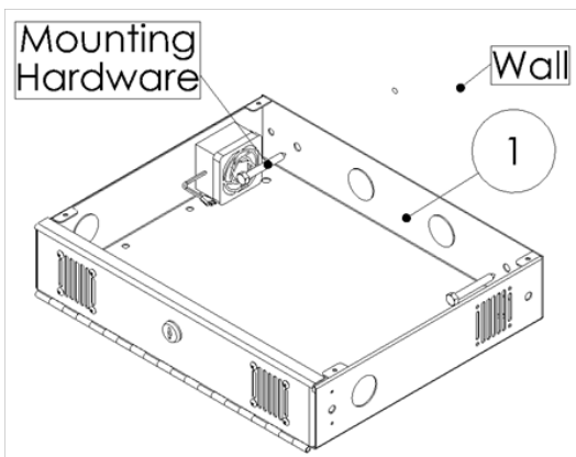
Step 9: Mounting the Bottom Box
