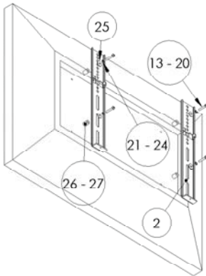
Step 3: Attaching the mounting brackets to the screen (spacers used due to recessed hole patterns)
