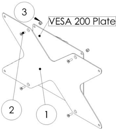
Step 2: Attaching the AP-1 to the mount
