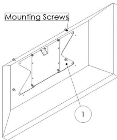
Step 3: Attaching the flat screen to the AP-1
