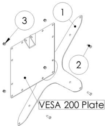
Step 2: Attaching the AP-2B to the mount
