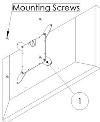
Step 3: Attaching the flat screen to the AP-2B
