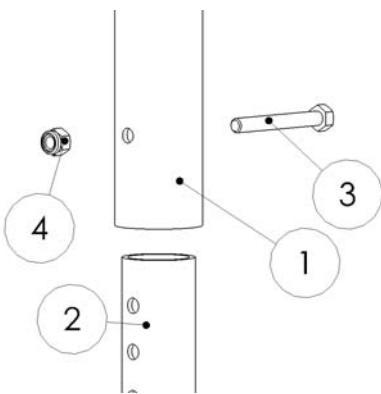
Step 4: Attaching the two masts
