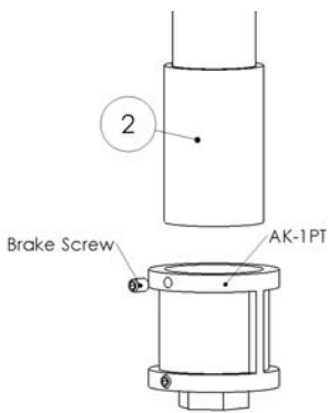
Step 2: Securing the outer mast
